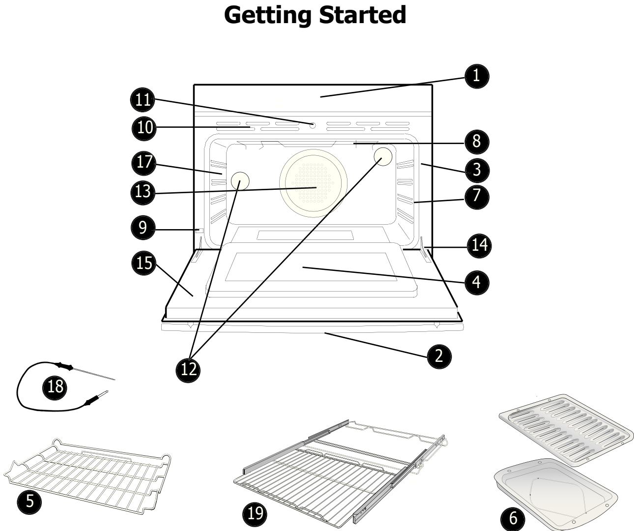
Figure 1: Oven Parts
